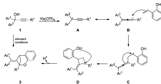
Scheme 4. Proposed Mechanism for the Formation of 3,4-Dihydro-2H-2,4-methanochromans
