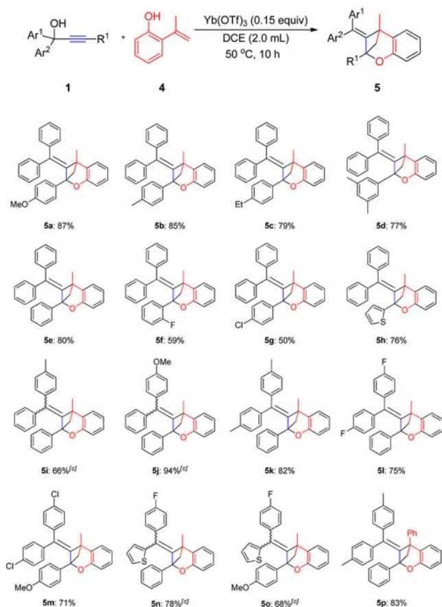
Scheme 2. Transformation of Propargylic Alcohols to 4-Methyl-3,4-dihydro-2H-2,4-methanochromans a-c
